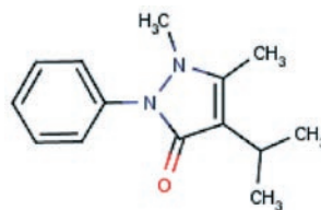
Slika 2. Strukturna formula propifenazona Figure 2. Structural formula of propiphenazone
