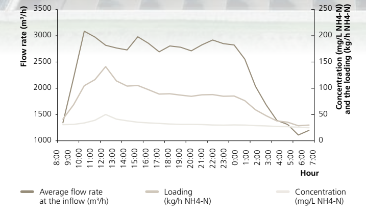
Flow rate at the inflow to CWWTP Ljubljana and the loading with ammonium nitrogen during the dry period between 22 August 2011 (8 a.m.) and 23 August 2011 (8 a.m.) Flow rates and the loading in wastewater increase in the morning and decrease during nighttime.
