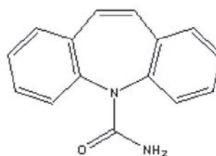
Slika 3. Strukturna formula karbamazepina Figure 3. Structural formula of carbamazepine
